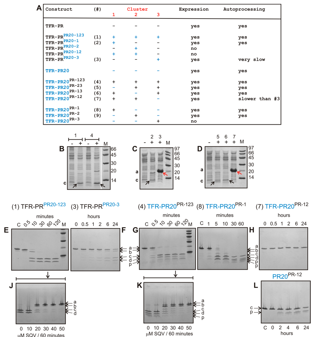
Figure 4. Expression and autoprocessing of TFR-PR precursors. (A) Identification of precursor constructs shown in panels B–I. Individual clusters and various combinations are shown with PR clusters in black and PR20 clusters in blue. (B–D) Expression and autoprocessing of precursor constructs containing one or more substituted clusters. Total cell extracts were analyzed by SDS–PAGE. Numbers above the lanes correspond to the designated construct shown in panel A, and lanes indicated by minus (–) and plus (+) represent total extracts of uninduced and induced cultures, respectively. (E–I) Time course of N-terminal autoprocessing of purified precursors in vitro . (F and I) TFR-PR PR20-3 and TFR-PR20 PR-12 exhibit very slow or no discernible autoprocessing, respectively, as indicated in panel A. (J and K) Inhibition of autoprocessing of TFR-PR PR20-123 and TFR-PR20 PR-123 conducted for 60 min in the presence of increasing concentrations of saquinavir. (L) Time course of autoproteolysis of mature PR20 PR-12 . Lowercase letters a–d and p indicate full-length precursor, an intermediate cleavage product of TFR-PR, TFR 9–56 -PR (cleavage occurs between residues 8 and 9 of TFR), mature PR, TFR, and products of mature PR autoproteolysis, respectively. The pathway to release the minor intermediate product TFR 9–56 -PR precedes the cleavage at the N-terminus of PR. We have shown previously that this cleavage is pH-dependent and becomes pronounced at pH 4. 2 M denotes molecular weight markers in kilodaltons. SQV denotes saquinavir.
