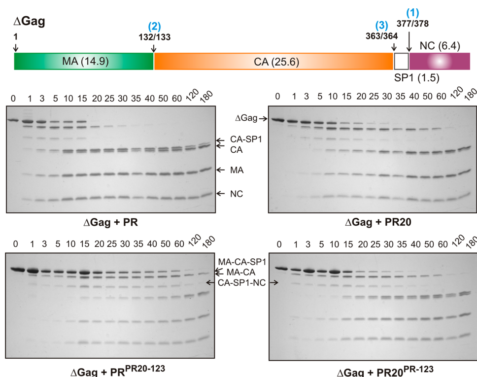
Figure 3. Processing of \Delta Gag by the protease. Schematic representation of the sequential cleavages of \Delta Gag with the order of cleavage (blue), cleavage-site positions, and calculated molecular weight (in kDa) of the products indicated. The four bottom panels show the time course of processing of \Delta Gag by mature protease monitored by SDS–PAGE on 18% Tris–glycine gels. Reaction mixtures contained 50 \mu M \Delta Gag and either 0.5 \mu M PR or 1 \mu M PR PR20-123 , PR20, and PR PR20-123 as indicated. Cleavage of full-length 48.4 kDa \Delta Gag between SP1 and NC (step 1) yields MA–CA–SP1 and NC, followed by cleavage between MA and CA (step 2) to generate the mature MA and the intermediate CA–SP1. The spacer polypeptide SP1 is cleaved subsequently (step 3) from the C-terminus of CA–SP1, some of which is still detectable just above mature CA at up to 180 min. No full-length \Delta Gag remains after reaction for 20 min with PR at half the concentration of the other three constructs, and no MA–CA–SP1 is detectable after 35 min. SP1, because of its small size, is predicted to have run out of the gel. A faint band between the MA–CA–SP1 and CA–SP1 bands corresponds to CA–SP1–NC formed by a minor MA/CA cleavage pathway.
