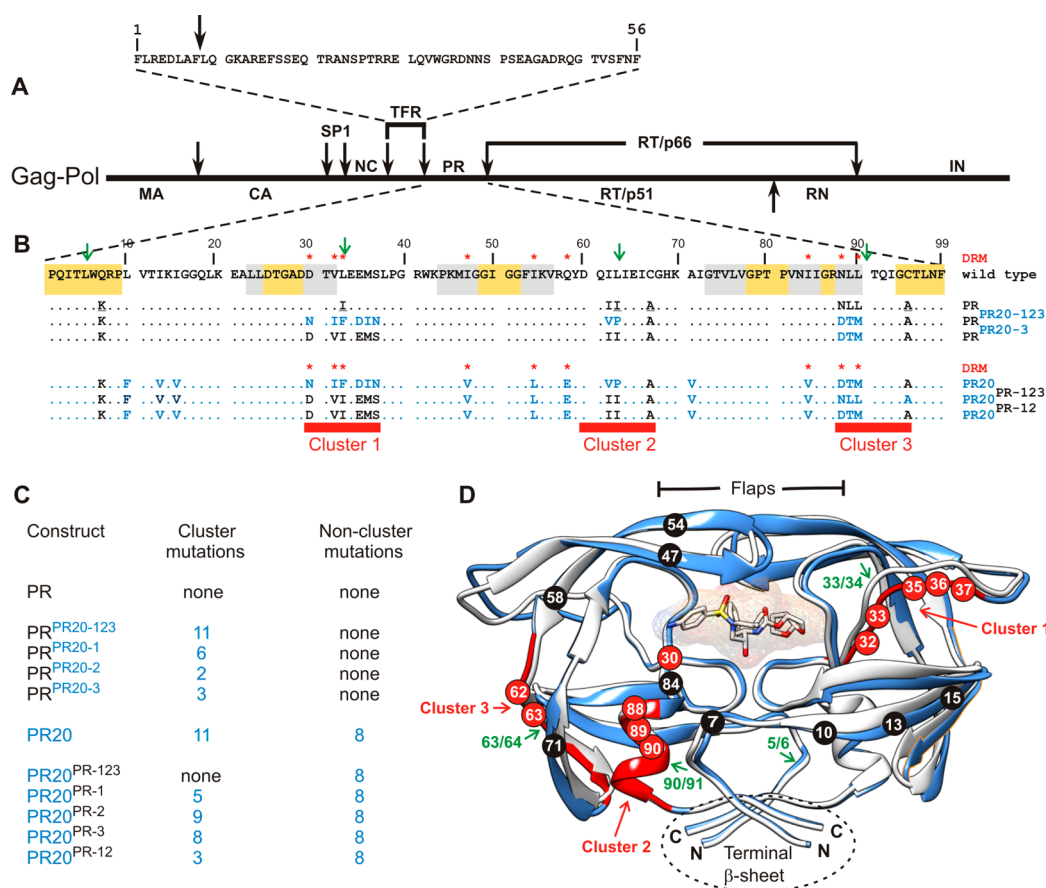
Figure 1. (A) Domain organization of the HIV-1 Gag-Pol polyprotein. Abbreviations: MA, matrix; CA, capsid; SP1, spacer peptide 1; NC, nucleocapsid; TFR, transframe region; PR, protease; RT, reverse transcriptase; RN, ribonuclease; IN, integrase. (B) Sequence alignment of wild-type protease, pseudo-wild-type protease (PR), and the multidrug resistant variant PR20. PR bears mutations Q7K, L33I, L63I, C66A, and C95A (colored black and underlined) to restrict autoproteolysis at sites indicated by green arrows and avoid cysteine-thiol oxidation. Introduced mutations common to PR and PR20 are Q7K, C67A, and C95A. The 19 mutations, both naturally occurring and selected under drug pressure, in PR20 are colored blue. Dots denote identical residues. Highly conserved regions in PR 52 are highlighted in yellow, and regions where major drug resistance mutations (indicated by red asterisks; http://hivdb.stanford.edu/cgi-bin/PIResiNote.cgi and ref 31) occur are highlighted in gray. The three clusters that contain mutations in PR20 next to sites of autoproteolysis in the wild type are indicated by red stripes. (C) List of PR, PR20, and derived mutants showing the number of cluster and noncluster mutations. (D) Superimposition of ribbon representations of PR20 in blue (PDB entry 3UCB) and PR in white (PDB entry 2IEN) bound to the inhibitor darunavir (stick representation) with the regions corresponding to the three clusters colored red as well as indicated by the red arrows corresponding to red stripes in panel B. Positions of mutations in cluster 1 (residues 30–37), cluster 2 (residues 60–67), and cluster 3 (residues 88–94) are labeled in white on red circles. The remaining eight of 19 mutations in PR20 are shown in white on black circles. Sites of autoproteolysis are denoted by the green arrows.
